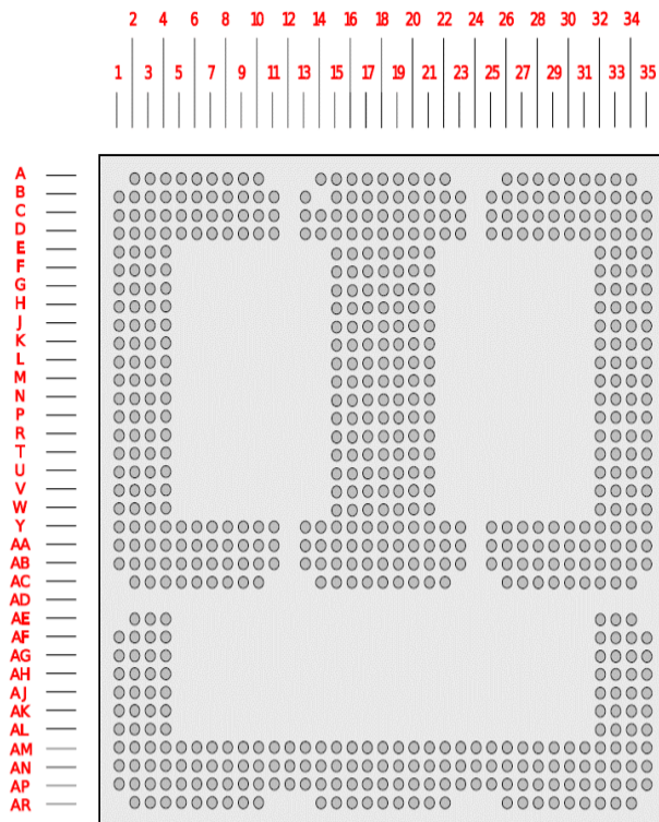
(Bottom View)
